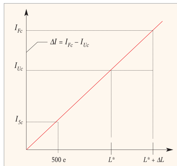
Fig. 2 The strain loading process
