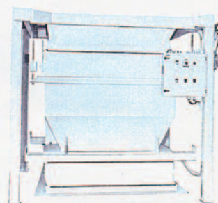
Receiving/shipping scales up to 10 000 kg Hopper scales for receiving and loading bulk goods
