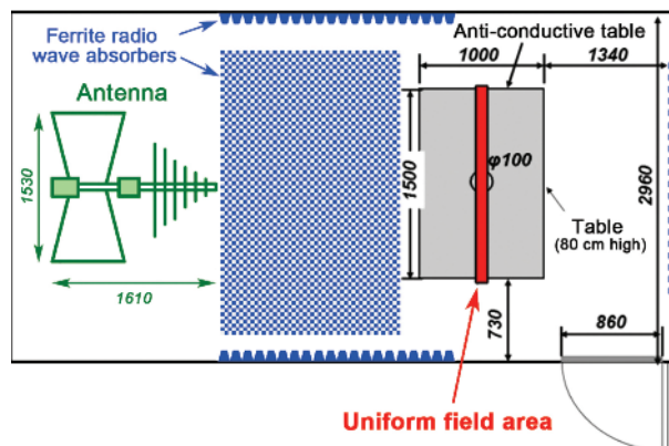
Figure 2 Horizontal layout of the equipment in the anechoic chamber
