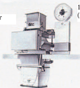
1883-2000: G balance. Here: G100 with residue weigher
