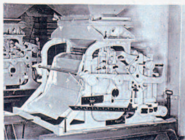
1883-2000: G balance. Here: G100 with residue weigher
