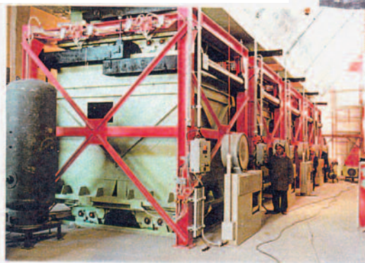
1981: 5 receiving/shipping scales 10 000 kg in Rio Grande
