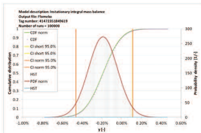
Figure 8: CDF and PDF as a function of the output estimate. The left vertical axis applies to the CDF, the right vertical axis to the PDF. The 95 % coverage interval is marked by two vertical lines.
