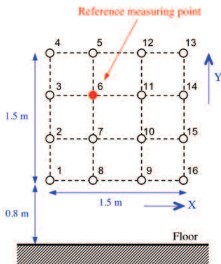
Figure 5 Two-dimensional arrangement of measuring points in the uniform field area (also see Figure 2). The EUT is placed in this area.
