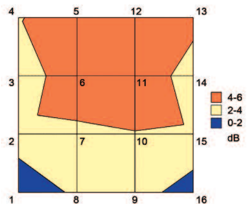
Figure 8 Two-dimensional distribution of field strength in the uniform field area at 500 MHz
