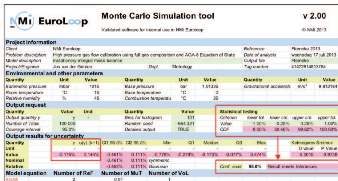
Figure 7: Dashboard of the Monte Carlo Simulator. The left red box contains the output estimate and the associated standard uncertainty. The top right hand box contains in the green cells the criteria and tolerances, the purple cells give the associated values of the CDF. The lower right hand box gives the result of the test based on the stated confidence level.
