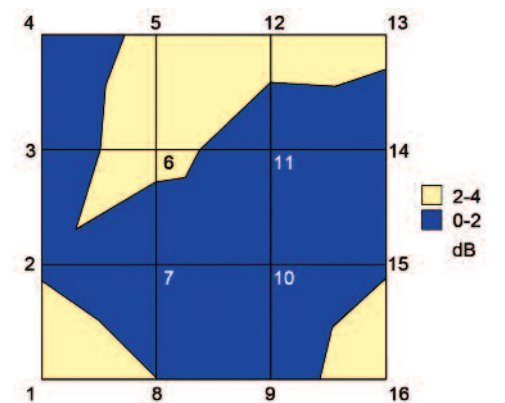
Figure 9 Two-dimensional distribution of field strength in the uniform field area at 2 GHz
