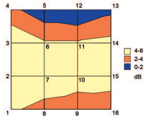
Figure 7 Two-dimensional distribution of field strength in the uniform field area at 26 MHz
