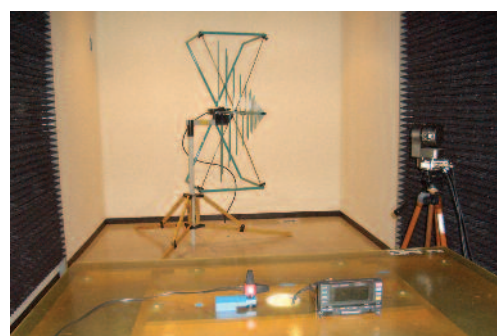
Figure 3 Inside the anechoic chamber with a table for the EUT and an antenna
