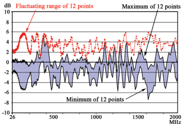
Figure 11 Maximum and minimum values and the magnitudes of fluctuating range of field strength at the 12 measuring points chosen according to the IEC standard
