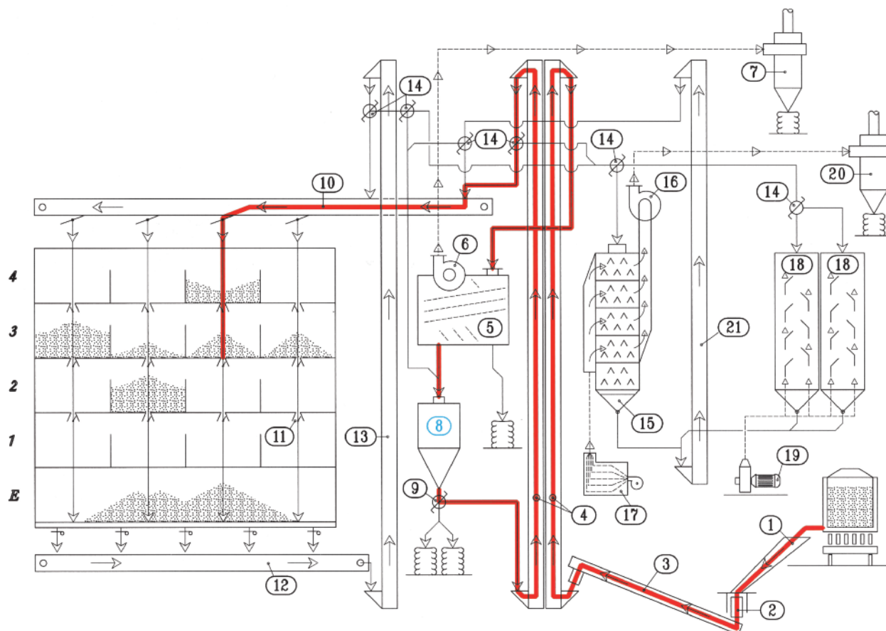
Function scheme of a flat-floor storehouse in Münster-Coerde. Diagram based on a figure from the Farwick-Mühlenbau company
