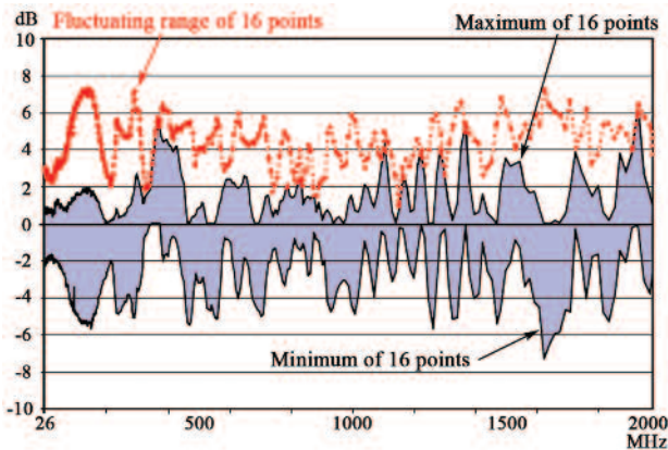
Figure 10 Maximum and minimum values of deviations of field strength at the 16 measuring points in the uniform field area at each frequency point
