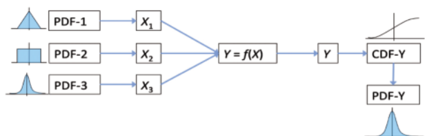
Figure 2 Schematic representation of the Monte Carlo process
