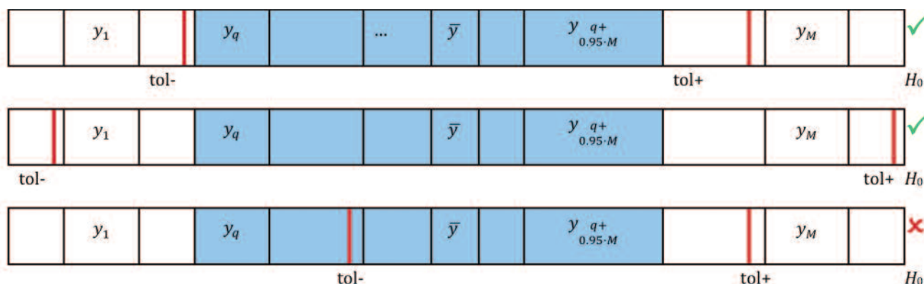
Figure 4: Tolerances (red lines) and coverage intervals around y (blue cells) while testing the null hypothesis H_0 . In the upper and middle rows the coverage interval is within the tolerances and H_0 is accepted. In the lower row the lower tolerance is in the coverage interval and H_0 is rejected.
