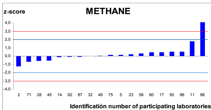
Figure 10 Results of the Bolivia proficiency test for methane
