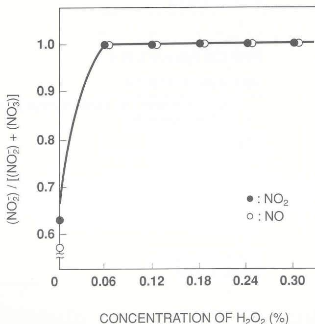
Fig. C Conversion of NO or NO_2 to NO_2^- versus concentration of H_2O_2 . Absorption solution: pH 13.0
