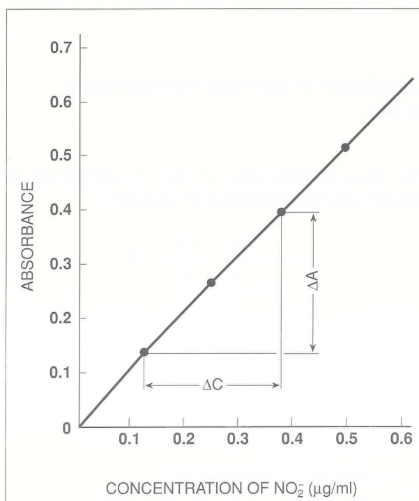
Fig. 4 An example of calibration curve for nitrogen oxides.
