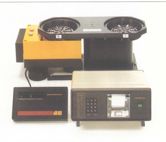
Fig. 2 Fully automatic mass comparator for testing mass standards up to 10 kg.
