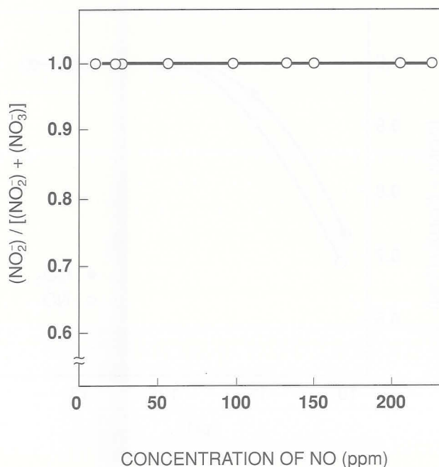
Fig. D Dependence of conversion of NO to \text{NO}_2^- on concentration of NO gas.
