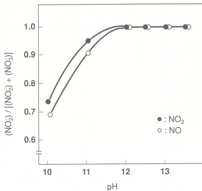
Fig. B Dependence of conversion of NO or NO_2 to NO_2^- on pH. Absorption solution: 0.15 % H_2O_2 .
