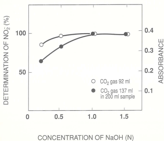
Fig. H Effect of \text{CO}_2 gas on the determination of \text{NO}_2^- at various concentrations of NaOH solution.
