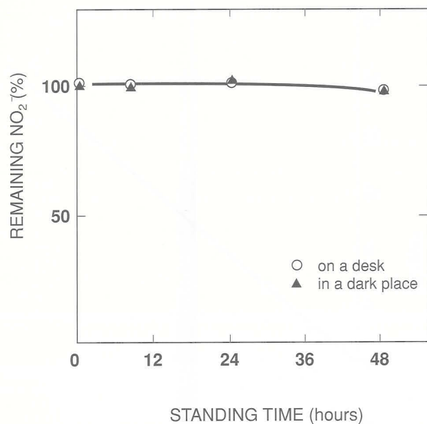
Fig. F Effect of standing time after the absorption of NO.
