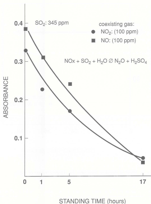
Fig. J Reaction of NO x with SO 2 in gas phase.
