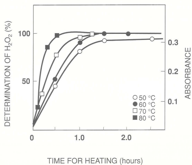
Fig. I Effect of temperature on the decomposition of \text{H}_2\text{O}_2 . Absorption solution: 2.0 % \text{H}_2\text{O}_2 .
