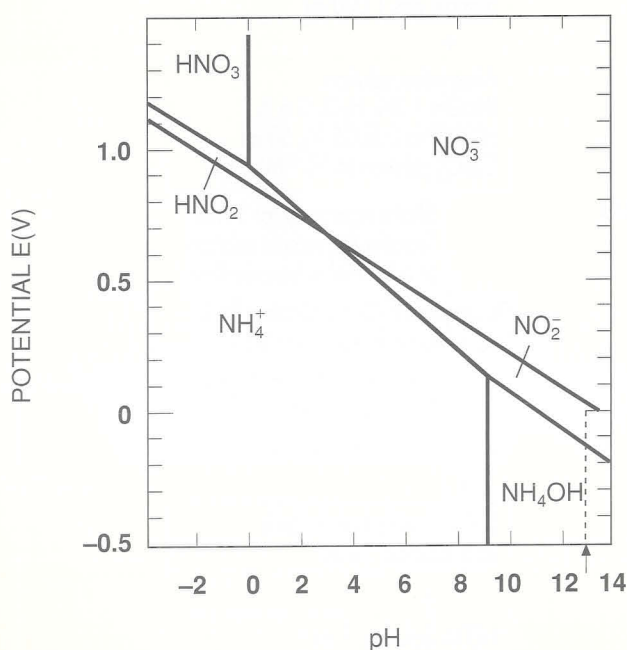
Fig. A Potential-pH (Pourbaix) – Diagram of the System N_2 - H_2O .
