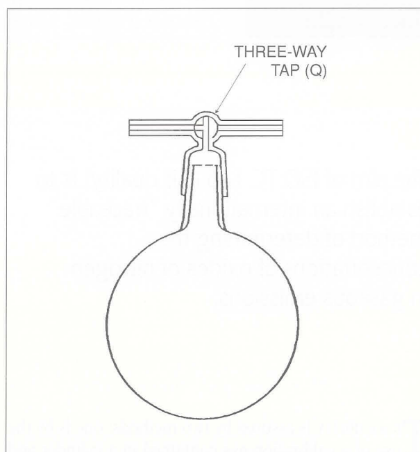
Fig. 1 Gas sampling flask (E) (Approximately 1 000 ml capacity)
