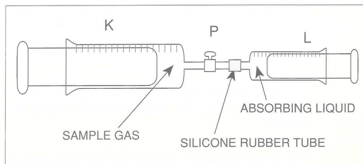
Fig. 2' Sampling syringe. The sample gas may be taken by means of a sampling syringe instead of the sampling flask. The capacity of the sampling syringe is 200 ml or 500 ml.
