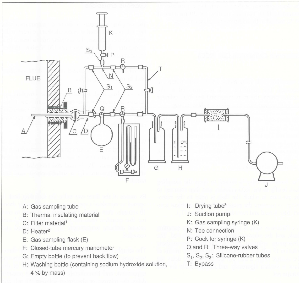
Fig. 3 Gas sampling apparatus.
