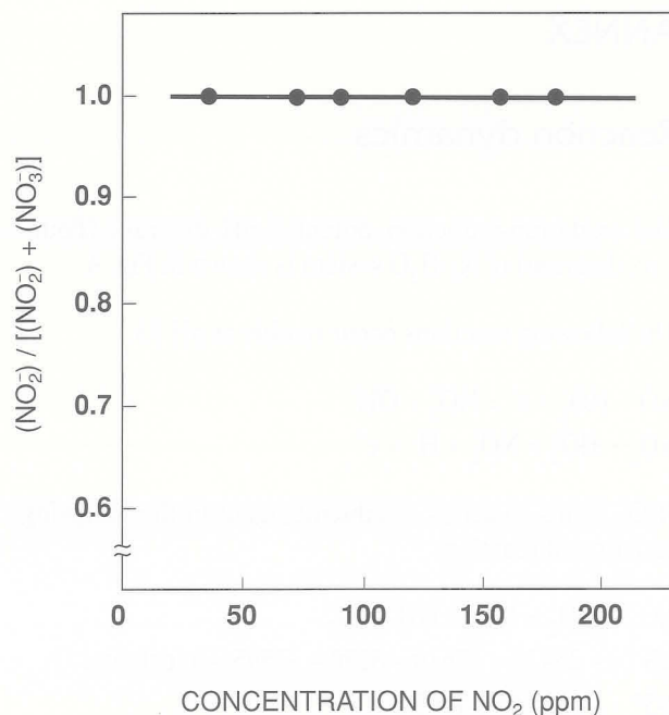
Fig. E Dependence of conversion of \text{NO}_2 to \text{NO}_2^- on concentration of \text{NO}_2 gas.
