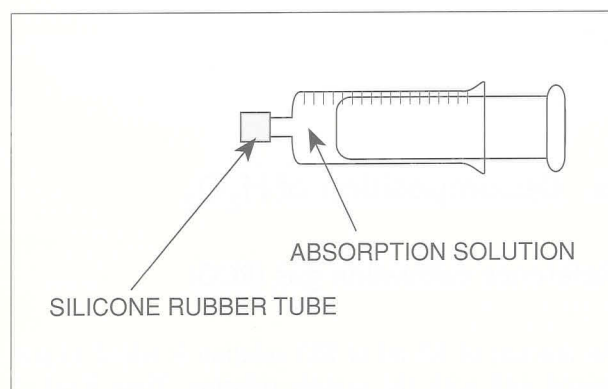
Fig. 2 Syringe for introducing the absorption solution.
