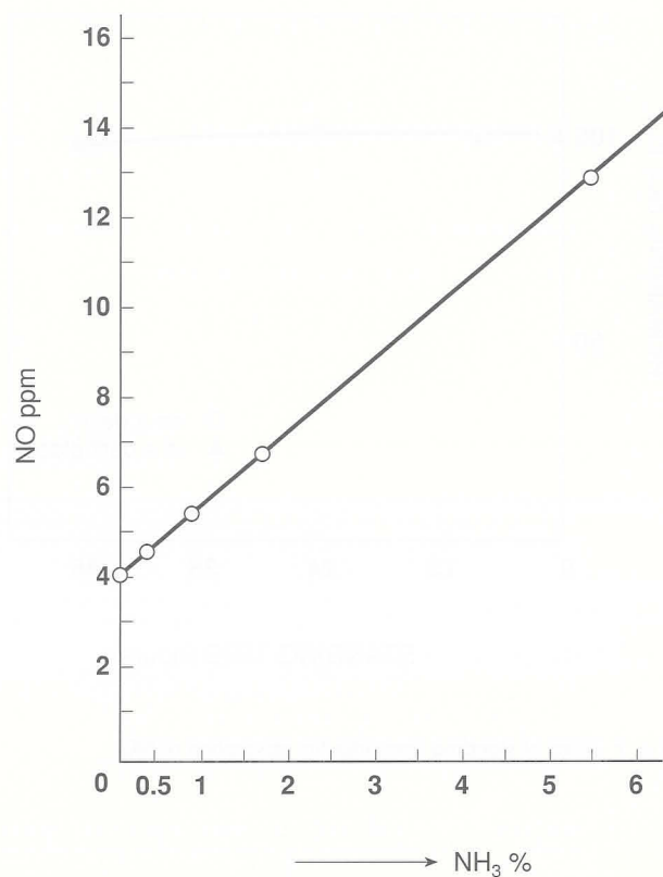
Fig. K Oxidation of NH 3 into N 2 O 5 by O 3 .
