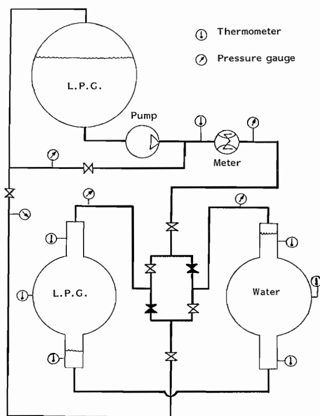
Fig. 4 — Calibration by double prover with water displacement
