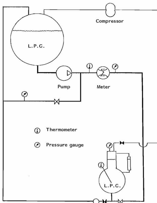
Fig. 2 — Calibration by "Bombola" type of closed prover
