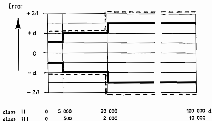
Fig. 1 — Maximum permissible errors for the verification of self-indicating weighing instruments with non automatic loading as a function of the load expressed in scale intervals d.
