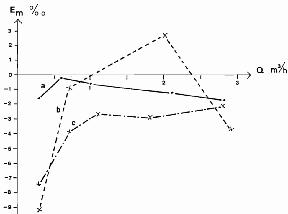
Fig. 3 — Results obtained with "Bombola" prover on measuring assembly No 55 989
